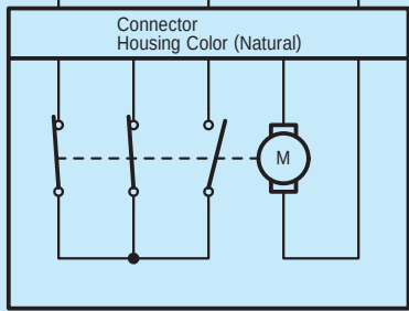
Damper Servo Motor (Rear Air Mix LH) (LHD) Damper Servo Motor (Rear Air Mix RH) (RHD)
