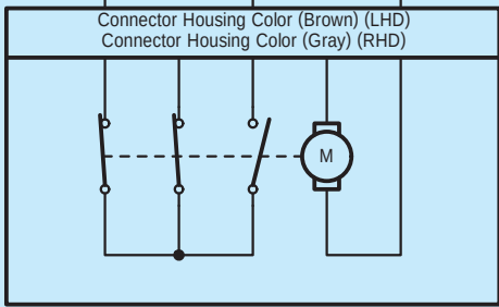
Damper Servo Motor (Rear Mode Control) (LHD) Damper Servo Motor (Cool Air) (RHD)
