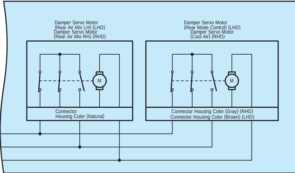
z66(C) A/C Blower Assembly
