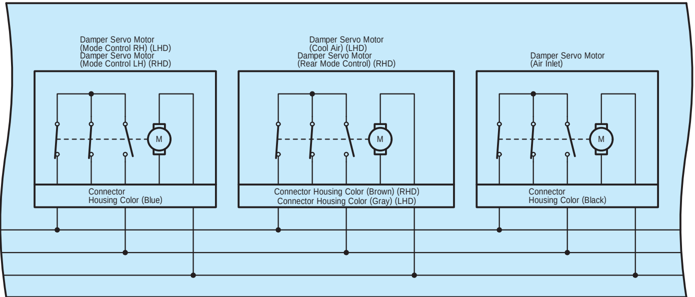
z66(C) A/C Blower Assembly
