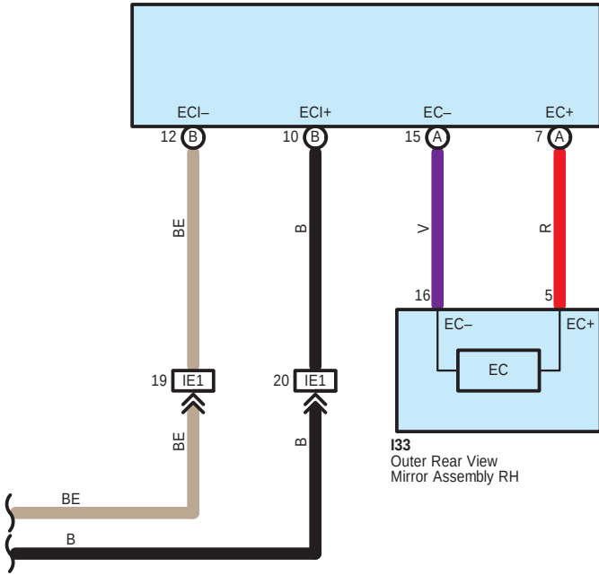
I37(A), I38(B) Outer Mirror Control ECU Assembly RH
