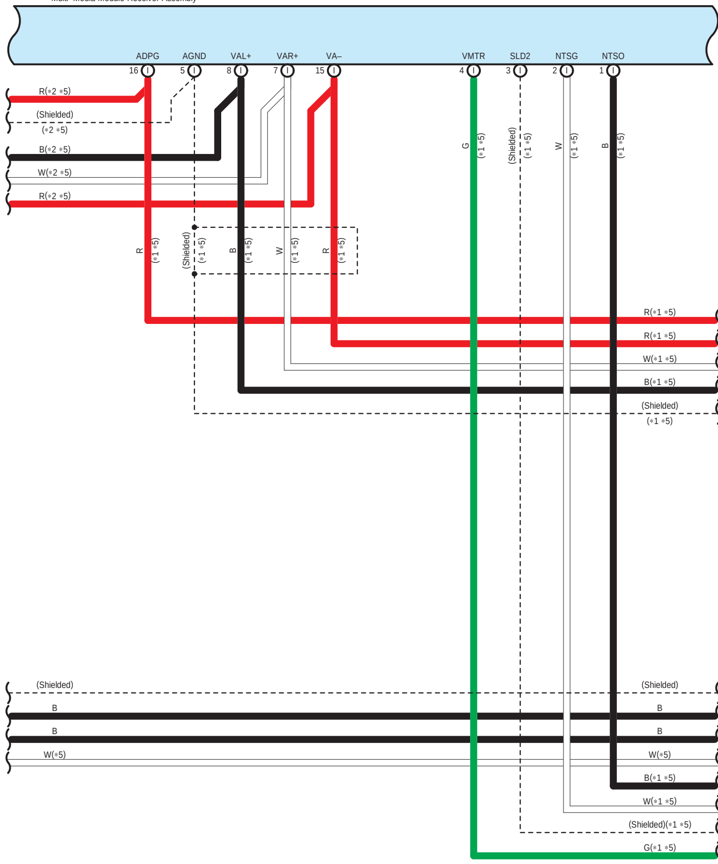
F76(H), F77(I), F80(M), F81(J), F85(L), F87(K) Multi-Media Module Receiver Assembly
