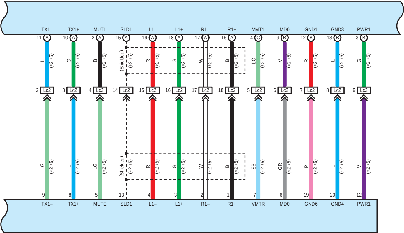
c60 Television Display Assembly RH
