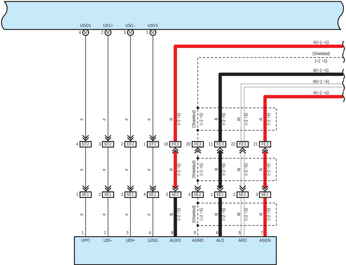
k1 No. 1 Stereo Jack Adapter Assembly
