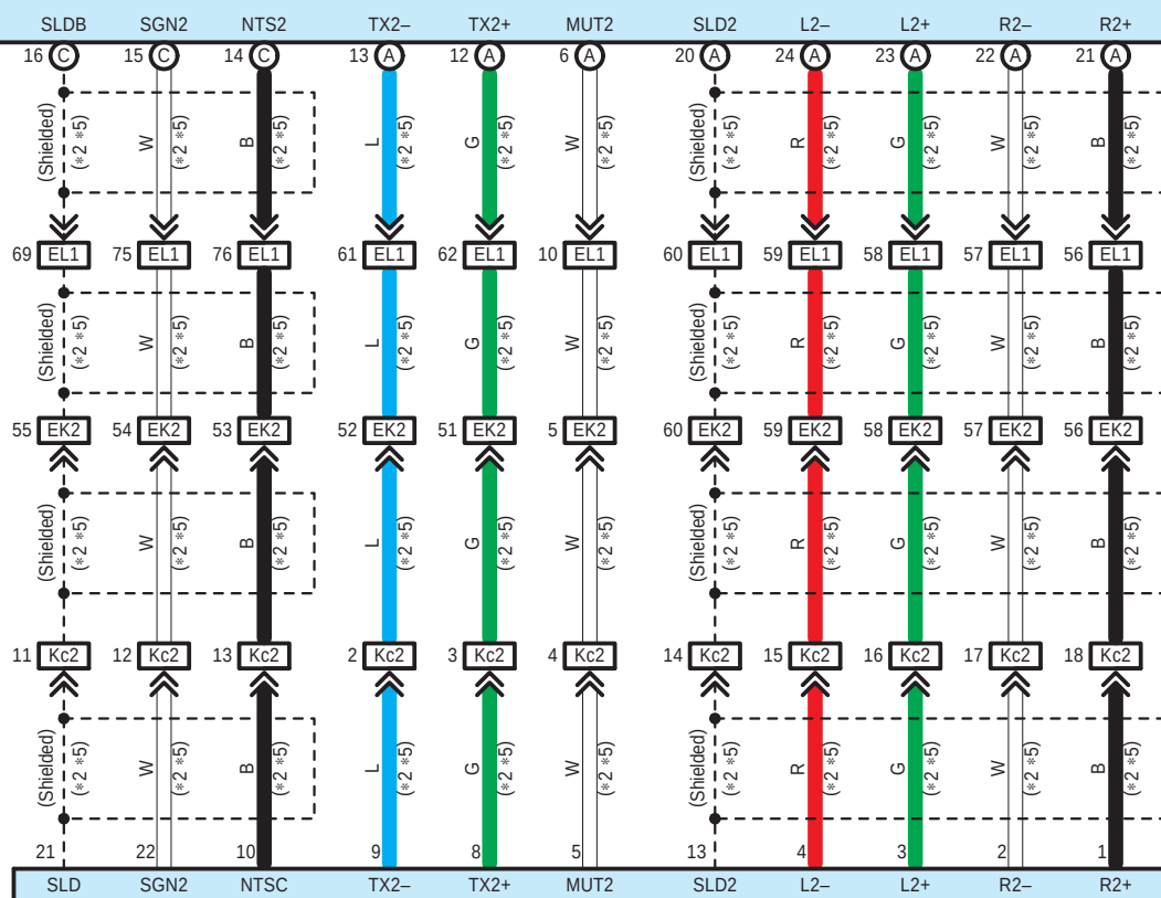
c61 Television Display Assembly LH
