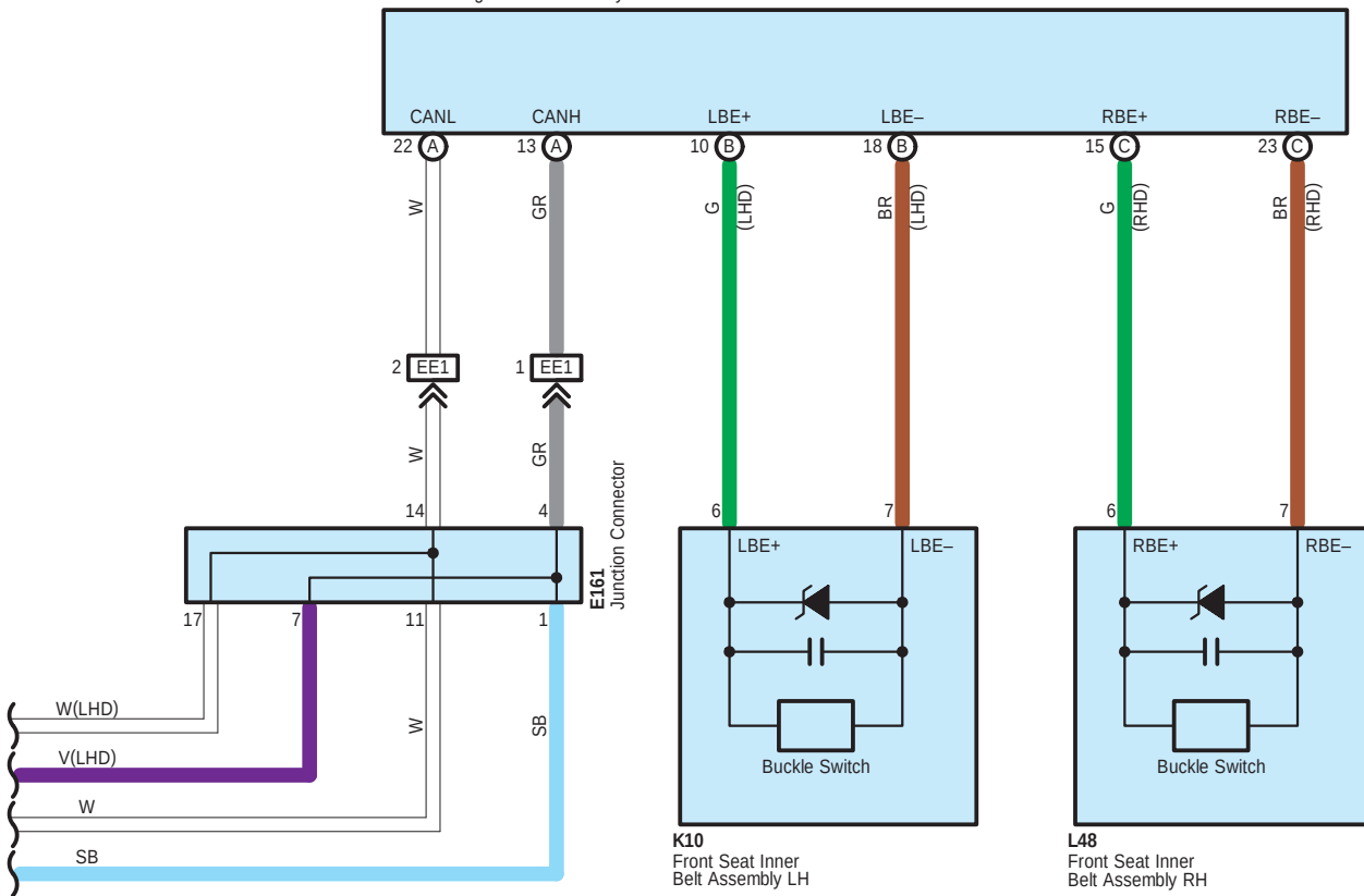
E47(A), K27(B), L27(C) Center Airbag Sensor Assembly
