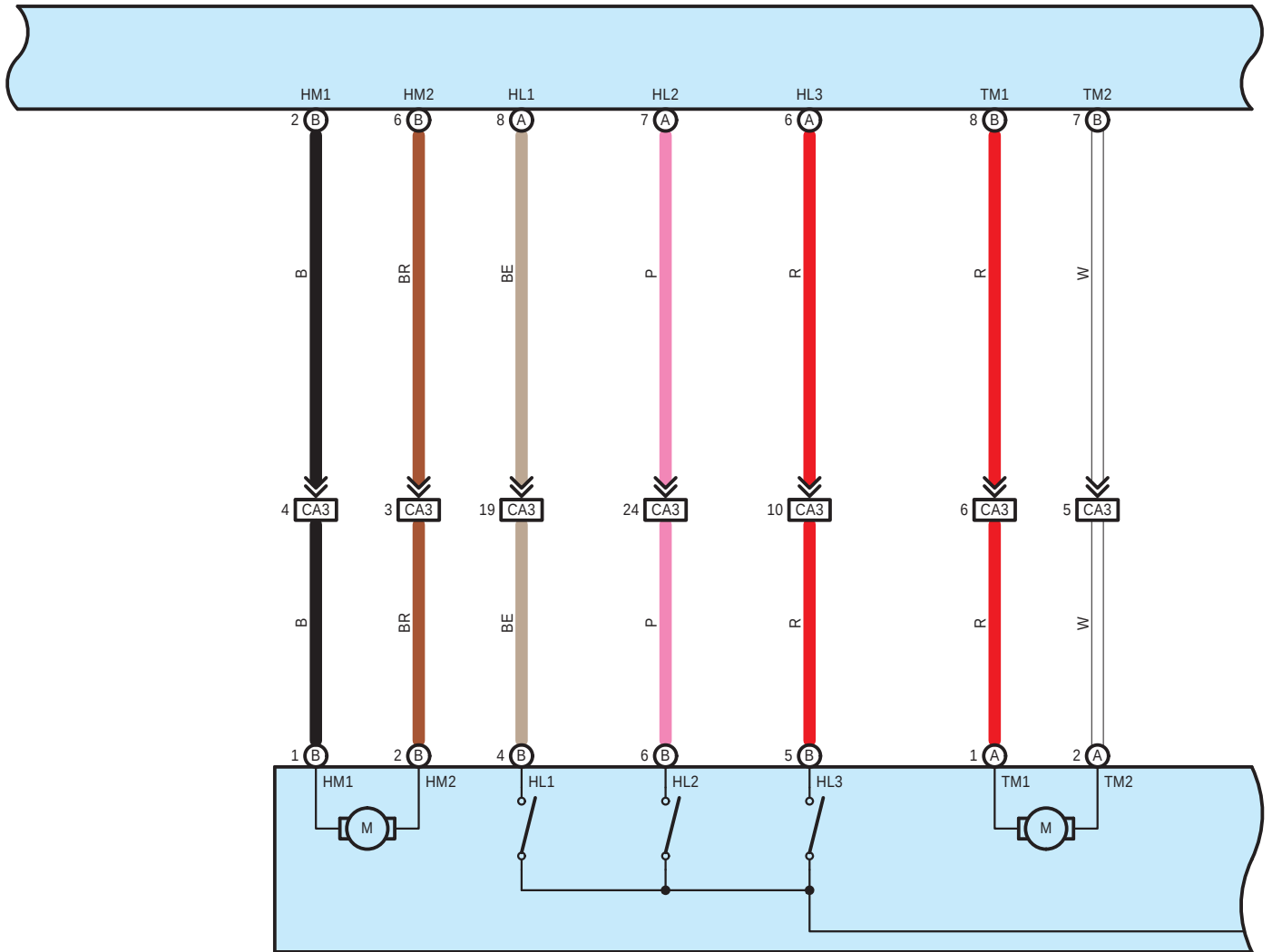
C43(A), C44(B), C49(C) Transfer Shift Actuator Assembly
