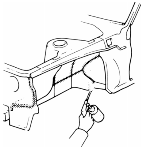
UNDERCOAT APPLICATION
