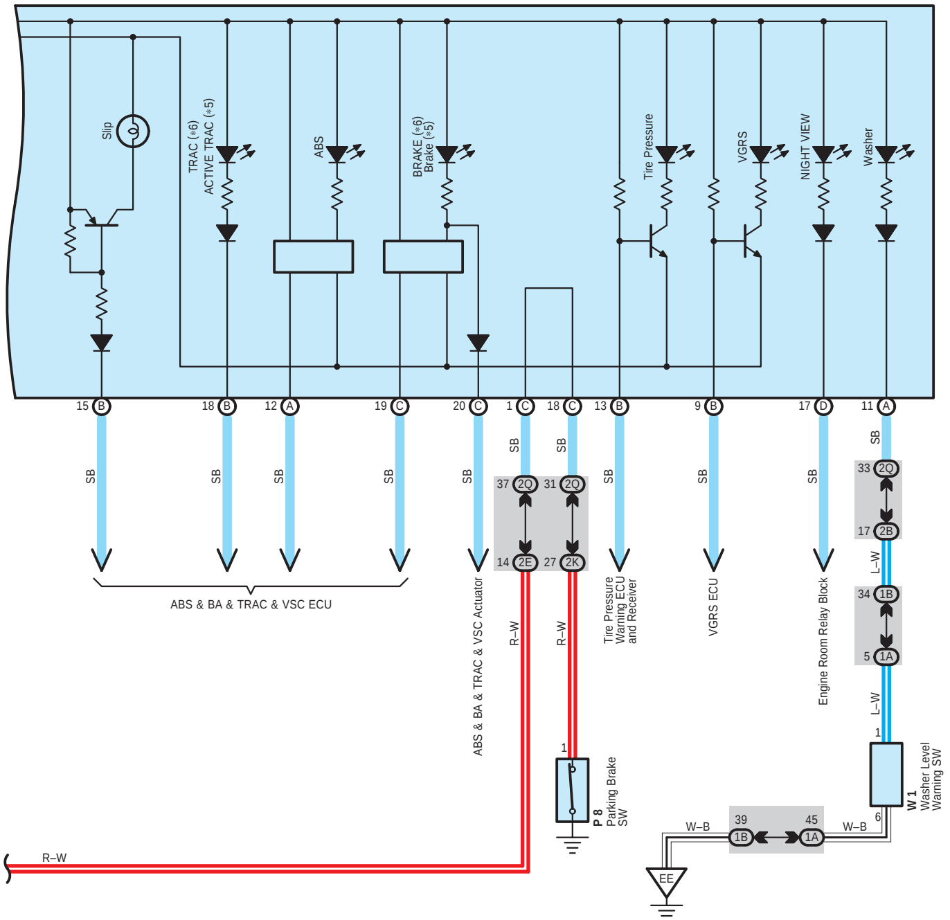
C14(A), C15(B), C16(C), C17(D) Combination Meter
