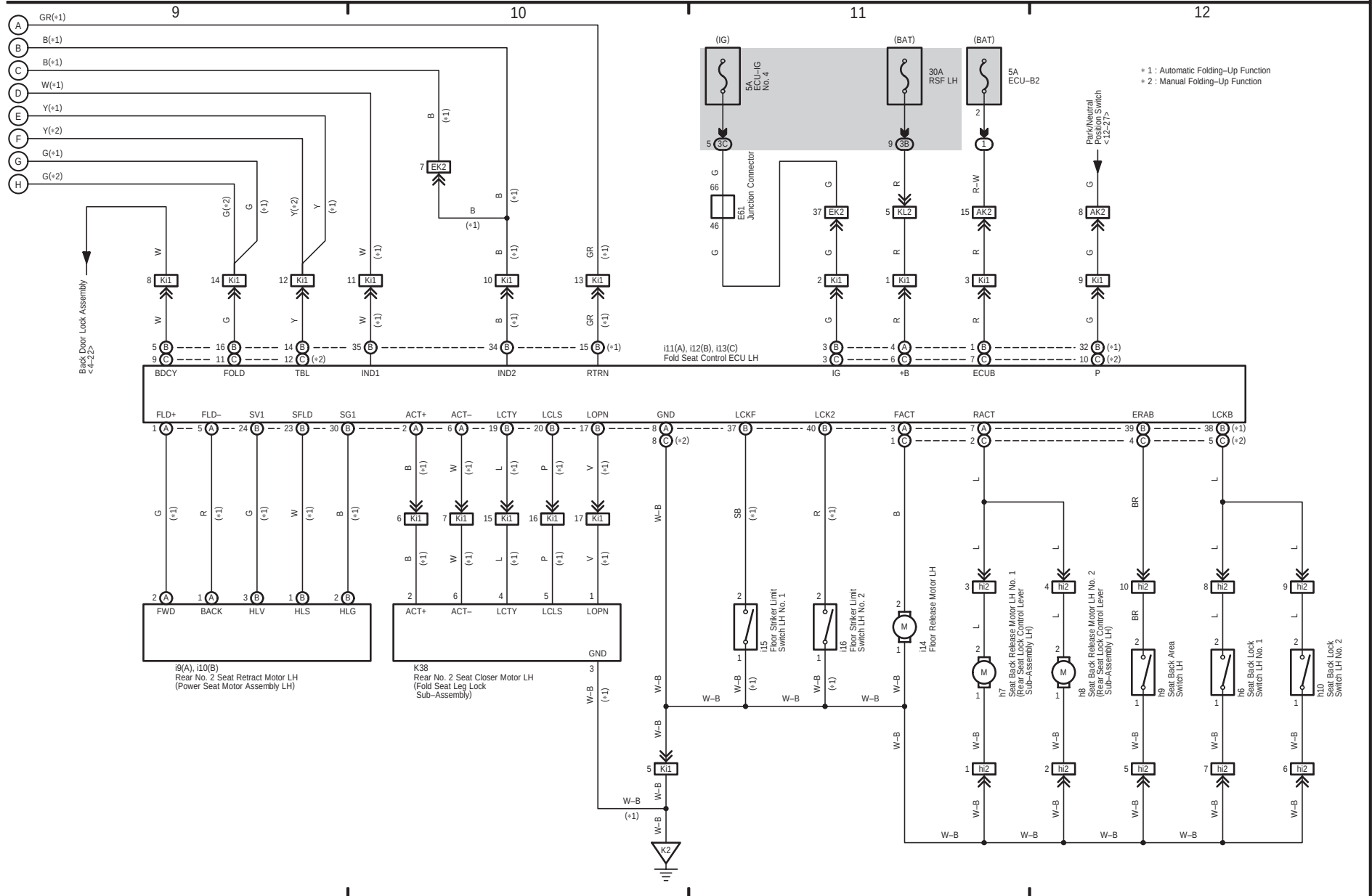
Rear Power Seat Control System (for Rear No. 2 Seat with Folding-Up Function)
