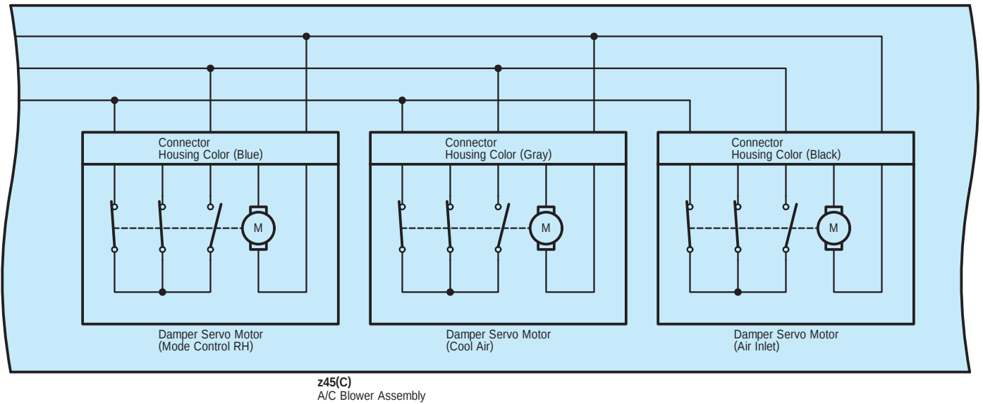
E35(A), E36(B), z45(C) A/C Amplifier Assembly
