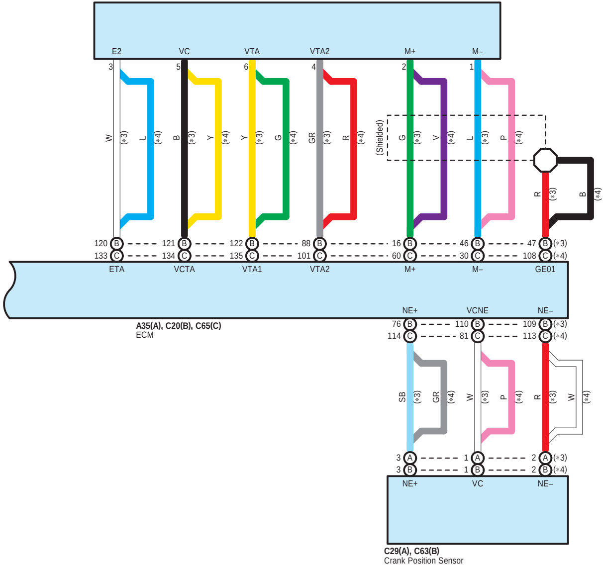
C2 Throttle Body with Motor Assembly
