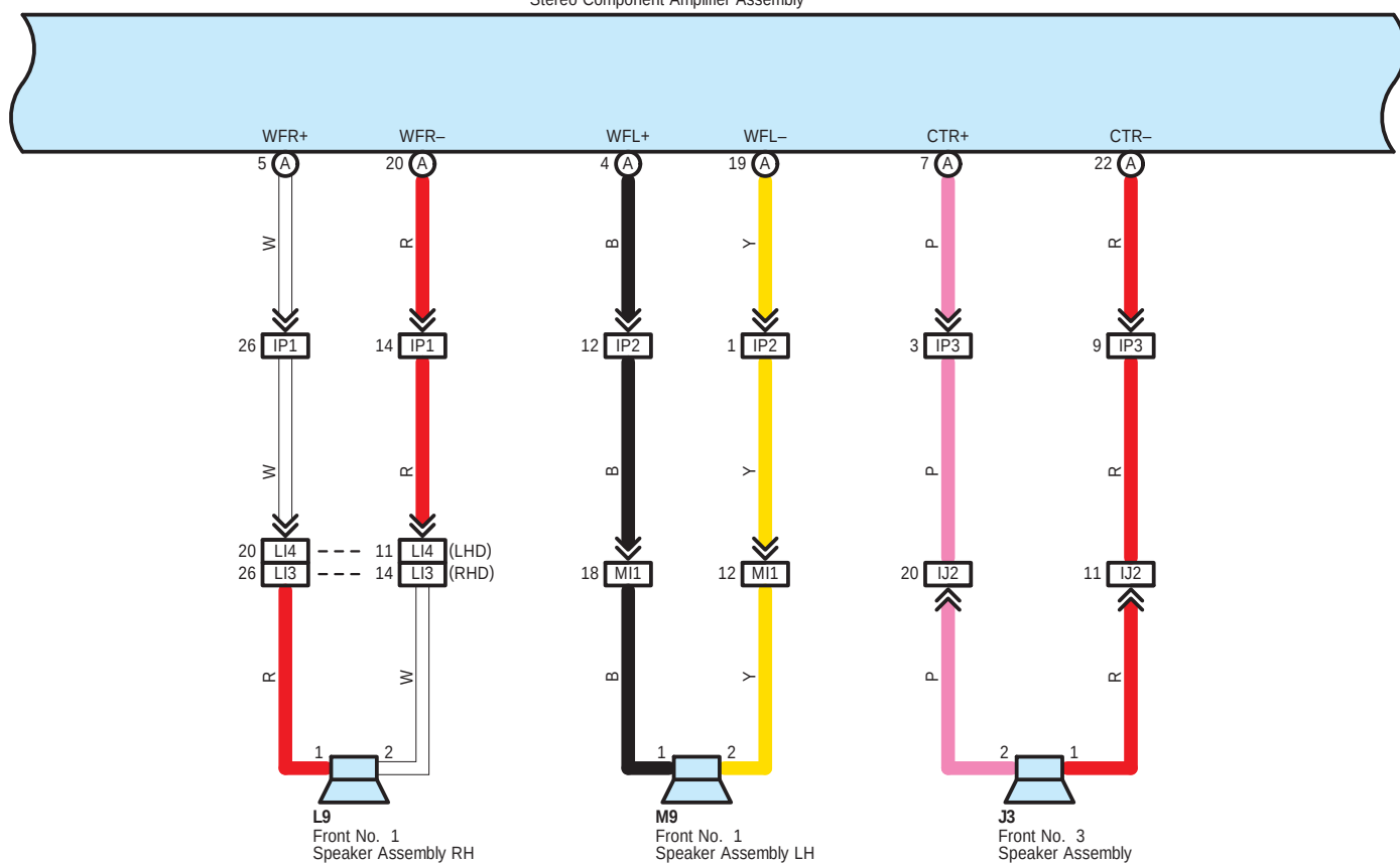
P22(A), P29(B) Stereo Component Amplifier Assembly
