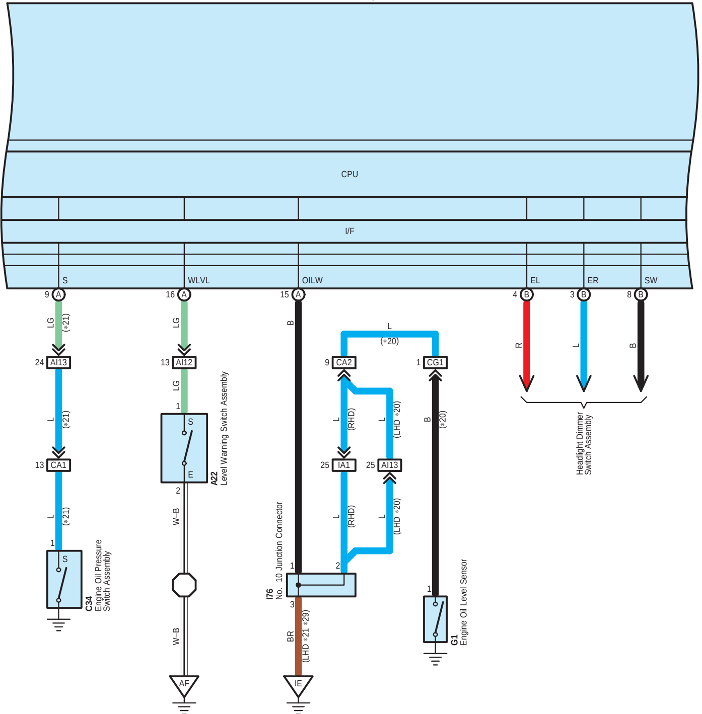
I10(A), I11(B), I105(C) Combination Meter Assembly
