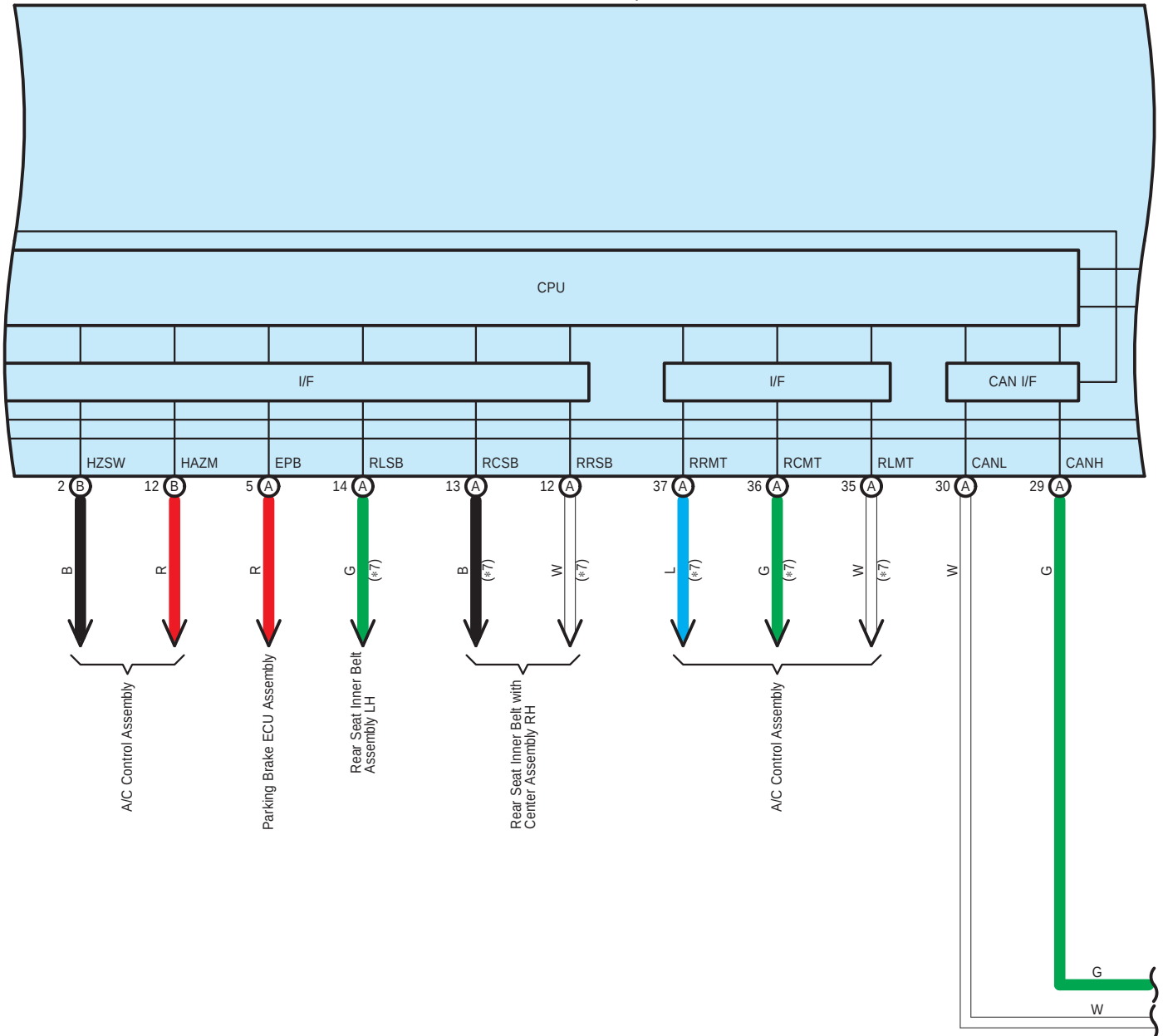
110(A), 111(B), 1105(C) Combination Meter Assembly
