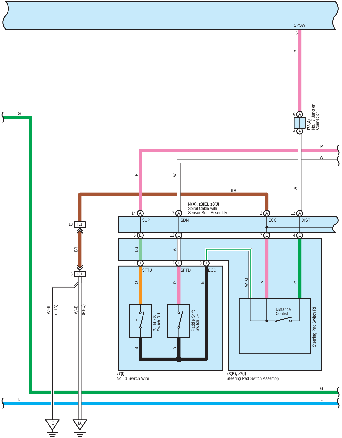
119 Driving Support ECU Assembly
