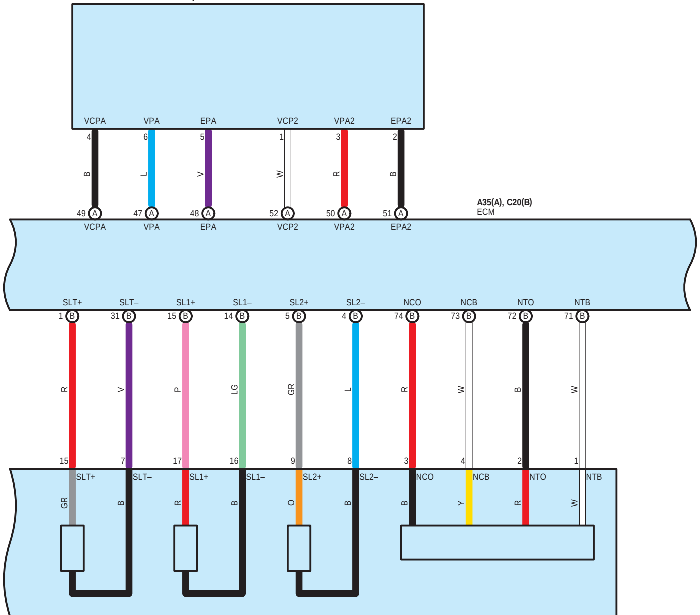
C21 Electronically Controlled Transmission Solenoid (Transmission Wire)
