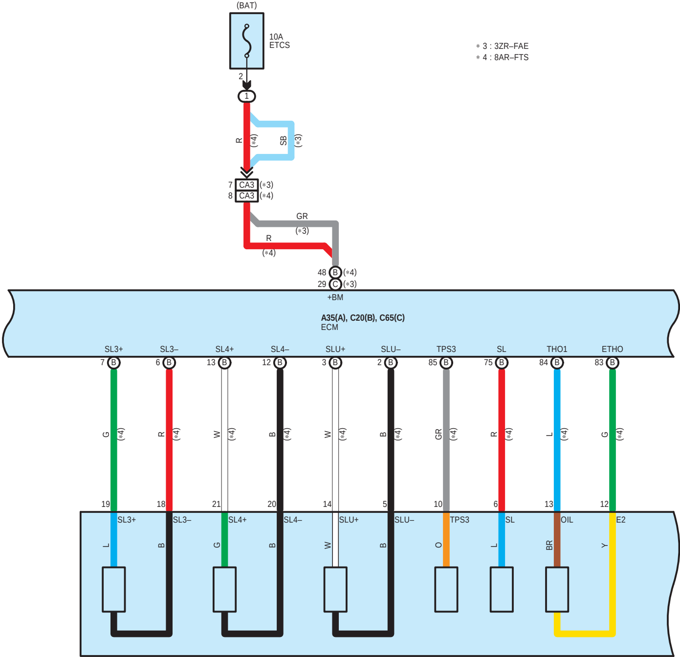
C21 Electronically Controlled Transmission Solenoid (Transmission Wire)
