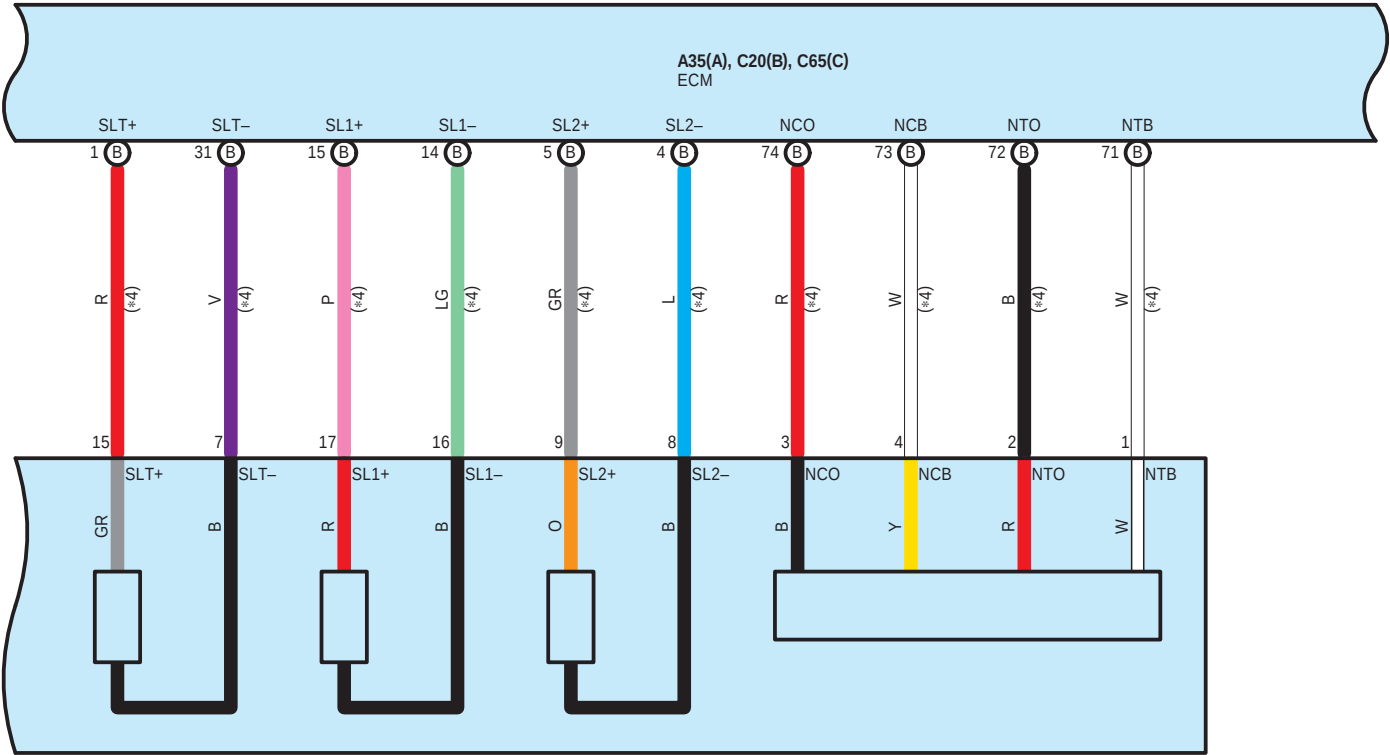
C21 Electronically Controlled Transmission Solenoid (Transmission Wire)
