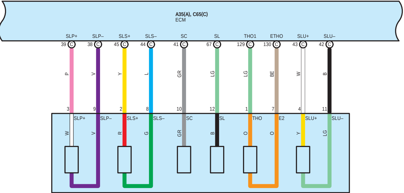
C49 CVT Solenoid (Transmission Wire)
