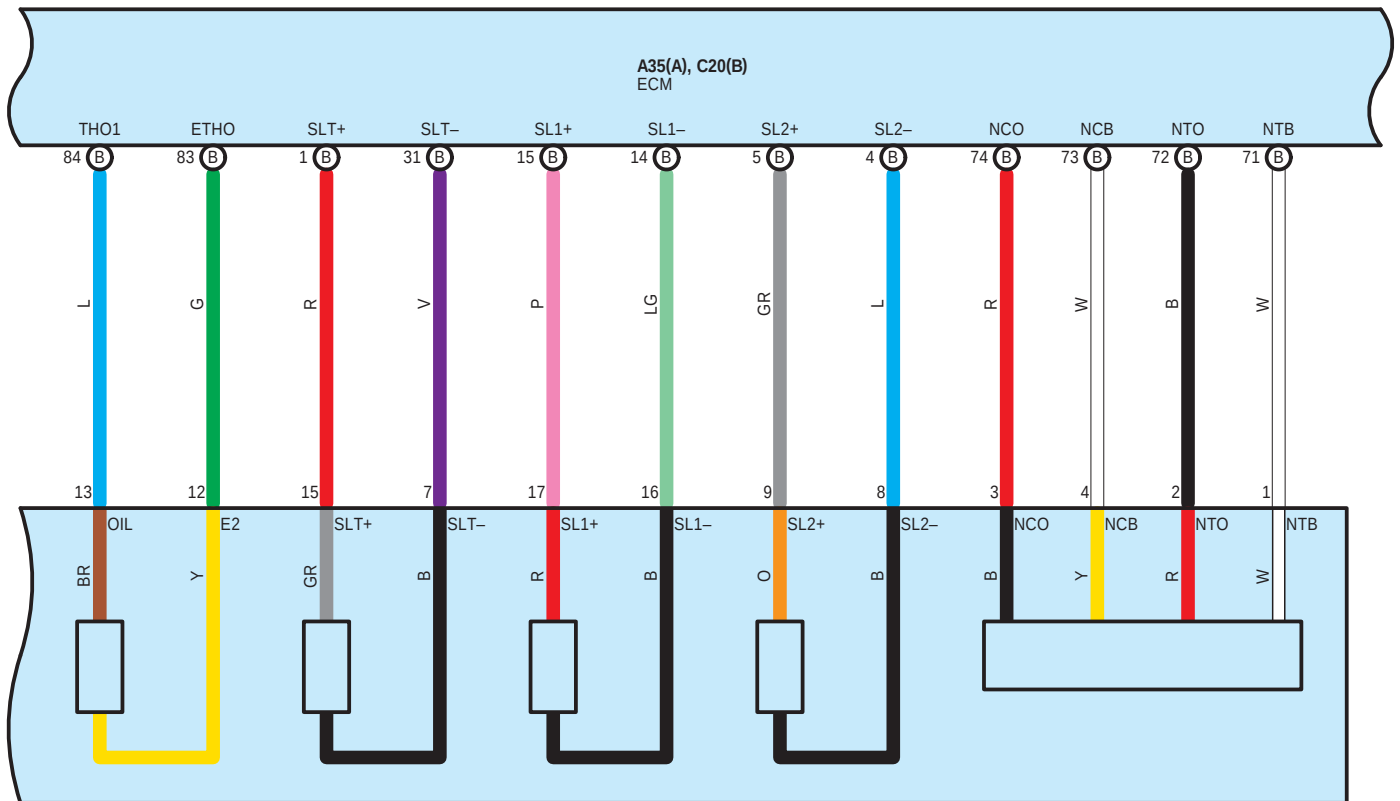
C21 Electronically Controlled Transmission Solenoid (Transmission Wire)
