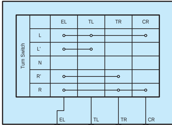
I31(A), I126(B) Headlight Dimmer Switch Assembly
