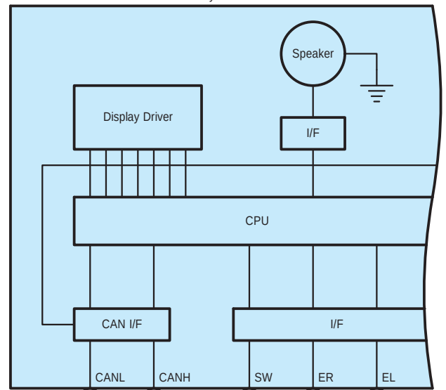
I10(A), I11(B) Combination Meter Assembly
