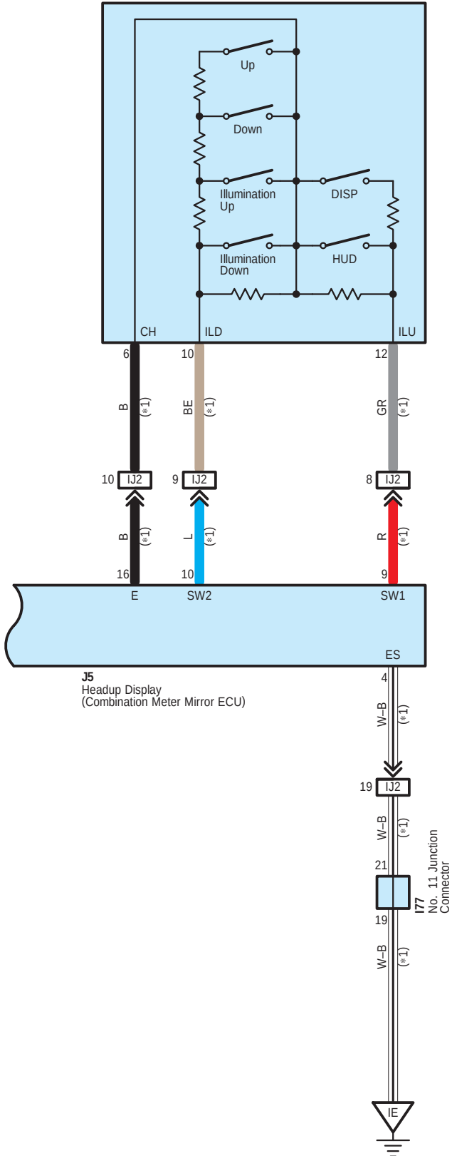
I70 Headup Display Switch Assembly
