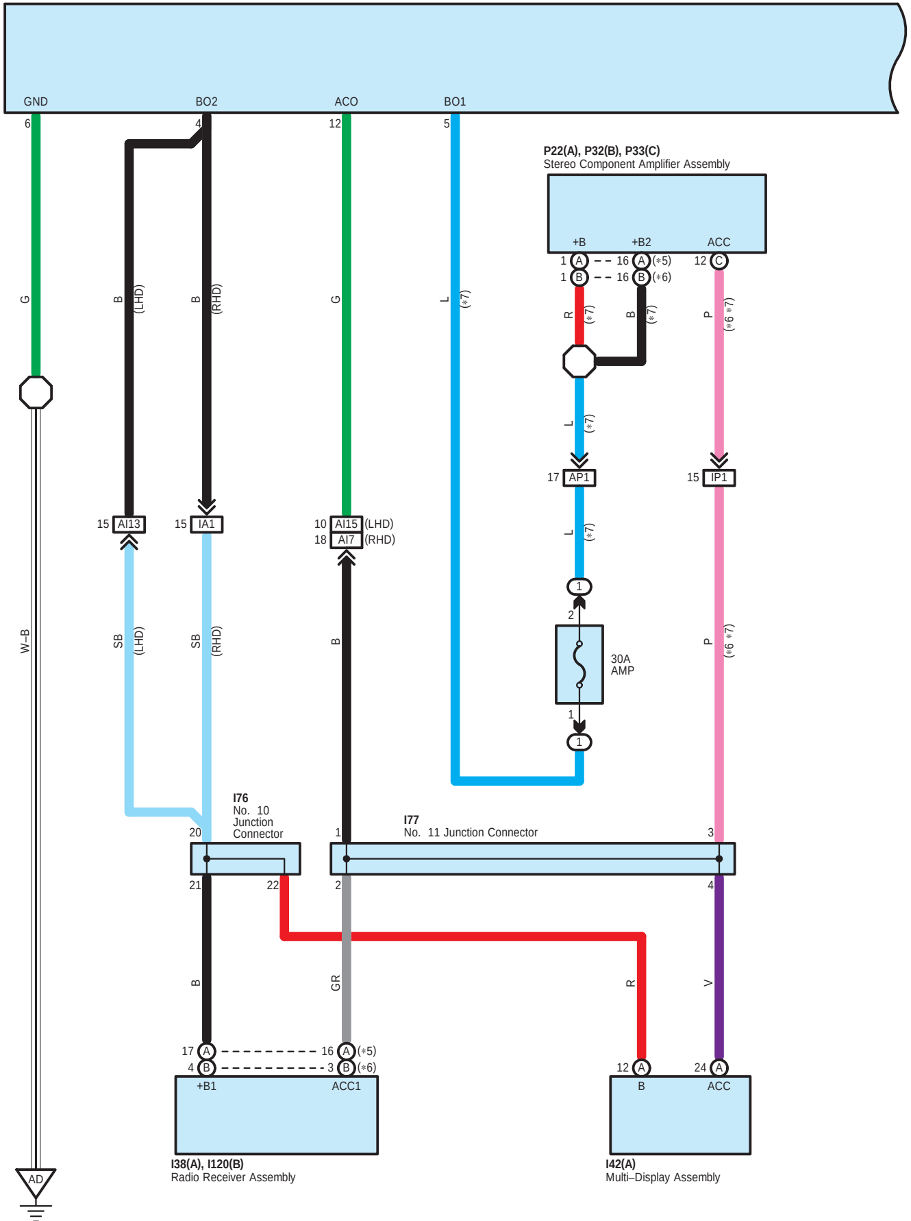
A8 Eco Run Vehicle Converter Assembly
