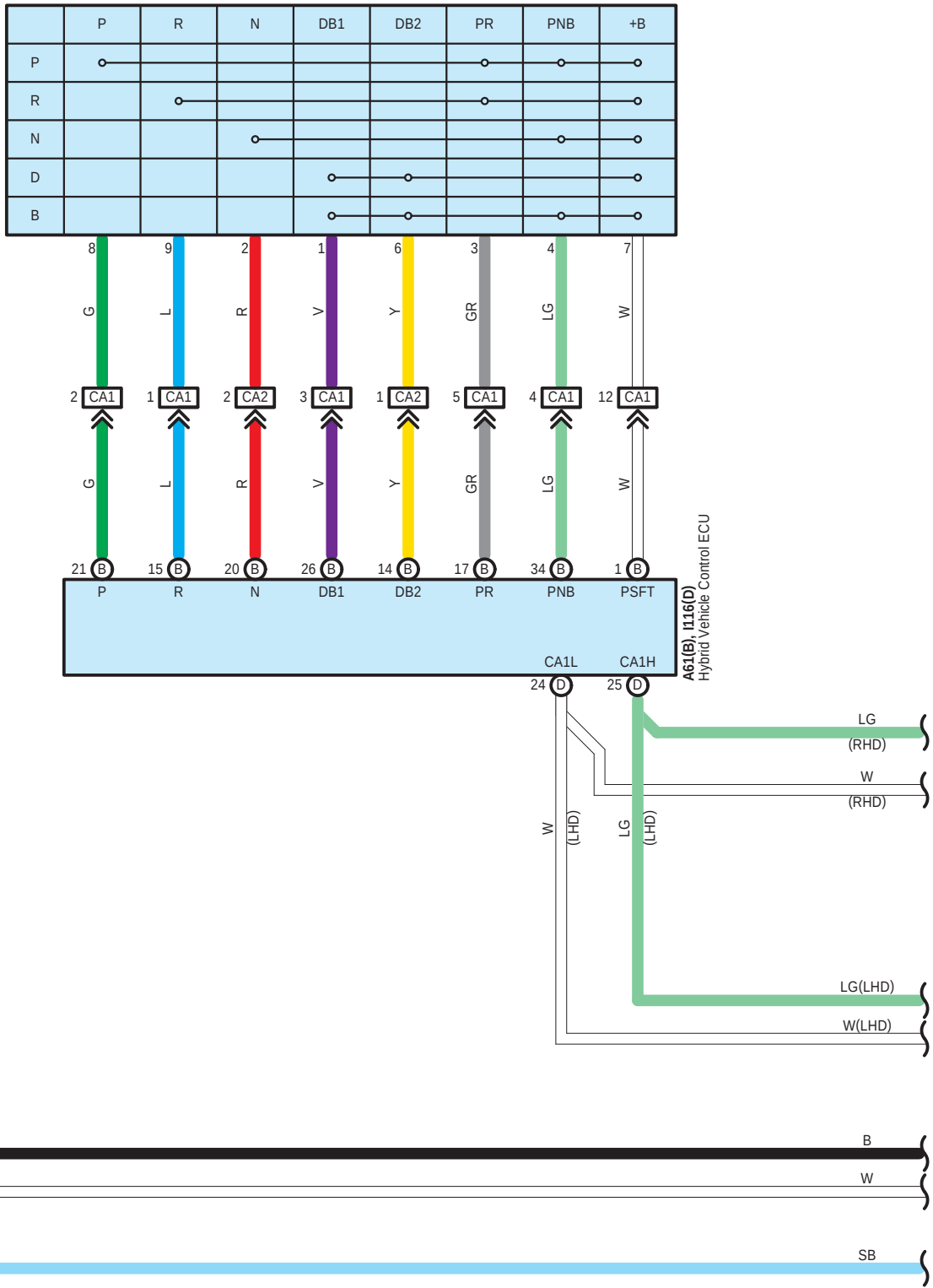
C42 Shift Lever Position Sensor
