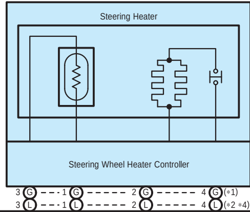
z6(G), z16(L) Steering Wheel Heater Control Assembly
