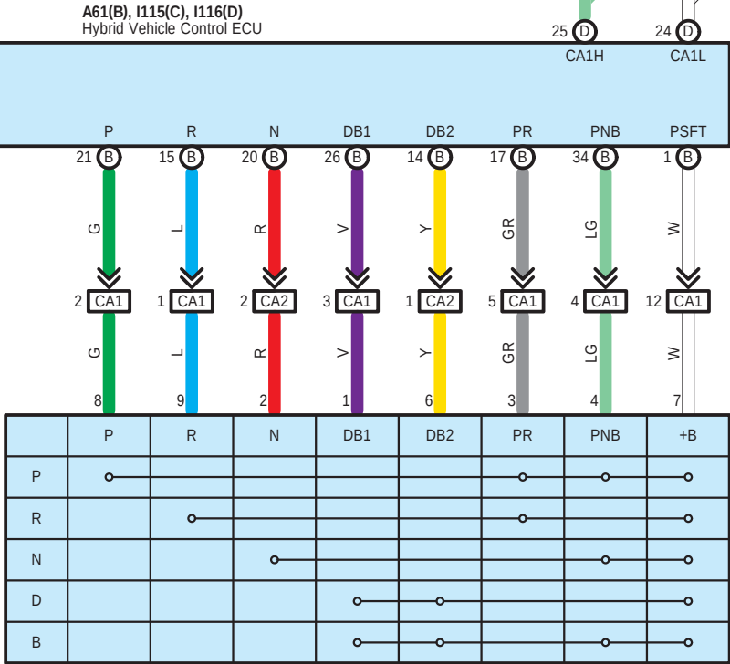
C42 Shift Lever Position Sensor
