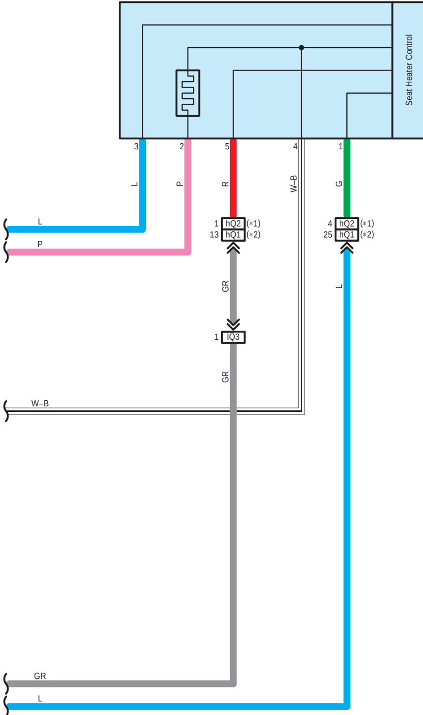
h7 Bench Type Rear Seat Back Cover RH
