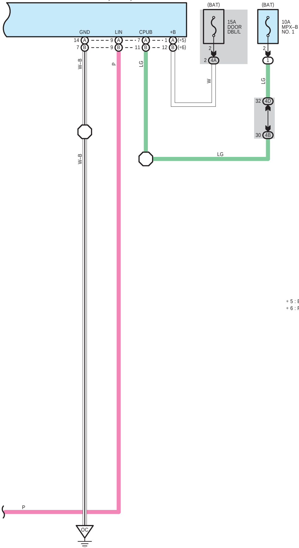
O41(A), O141(B) Double Lock Door Control Relay Assembly
