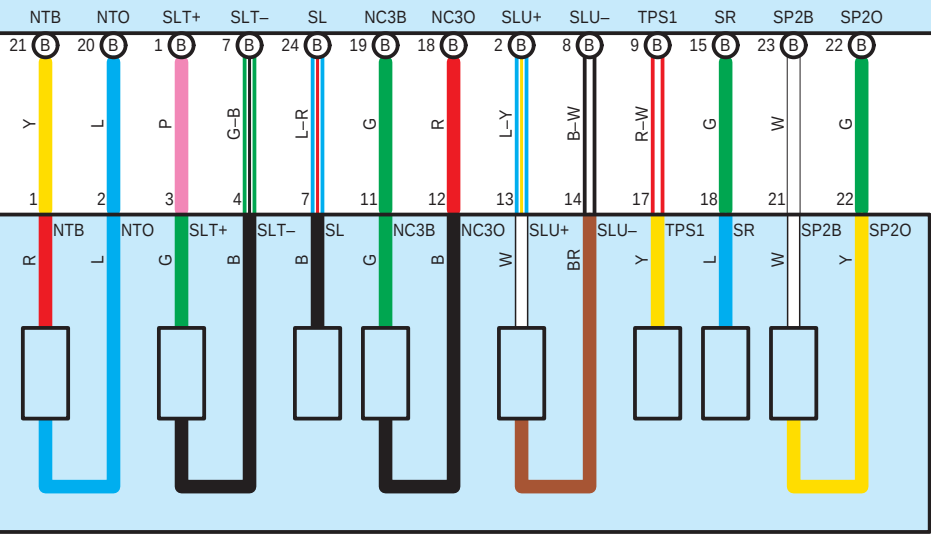
F25 ECT Solenoid (Transmission Wire)
