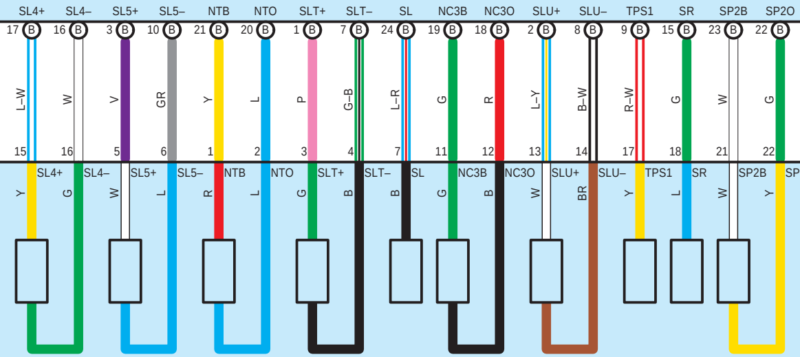
F25 ECT Solenoid (Transmission Wire)
