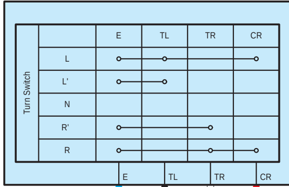
O22 Headlight Dimmer Switch Assembly
