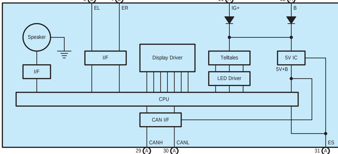
O3(A), O4(B) Combination Meter Assembly
