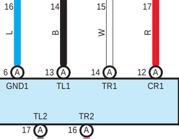
O23(A) Windshield Wiper Switch Assembly
