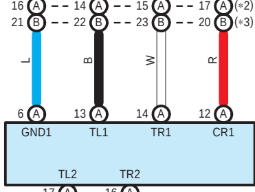
O23(A) Windshield Wiper Switch Assembly
