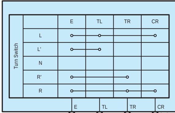
O22(A), (B) Headlight Dimmer Switch Assembly
