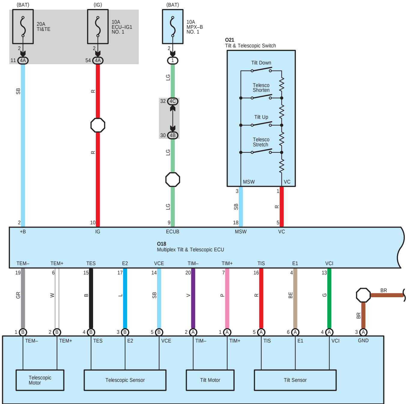
O19(A), O20(B) Tilt Steering Gear with Motor Assembly
