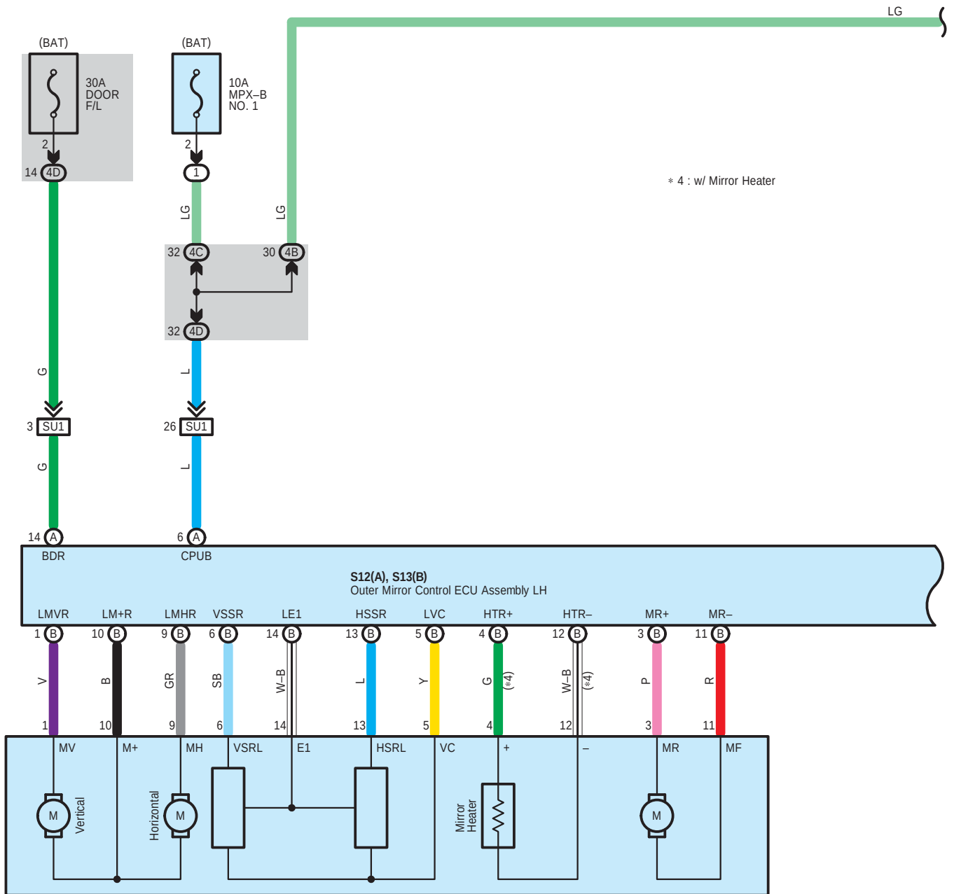
S7 Outer Rear View Mirror Assembly LH
