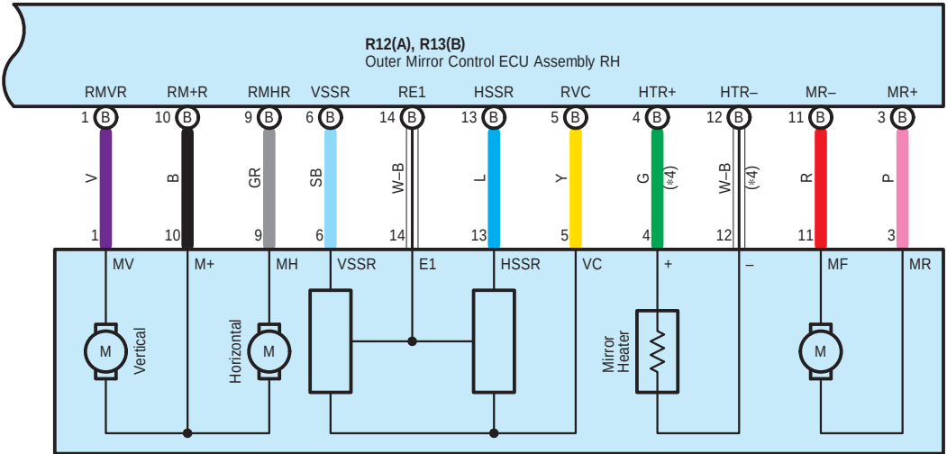
R7 Outer Rear View Mirror Assembly RH
