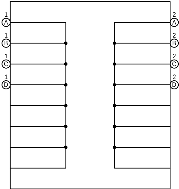
O171(A), O172(B), O173(C),O174(D) No. 12 CAN Junction Connector
