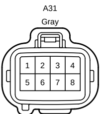
90980-10897 (Headlight)
