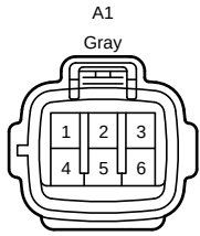
90980-11194 (Front Turn Signal Light, Headlight Leveling Motor)
