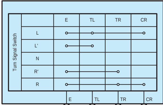
O22(A) Headlight Dimmer Switch Assembly
