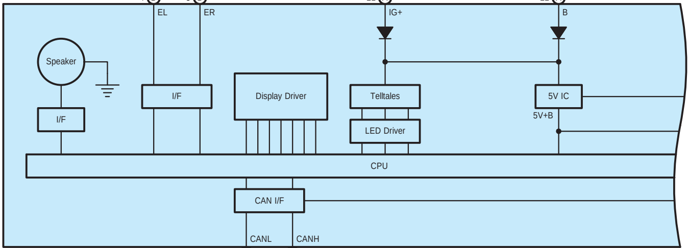
O3(A), O4(B) Combination Meter Assembly
