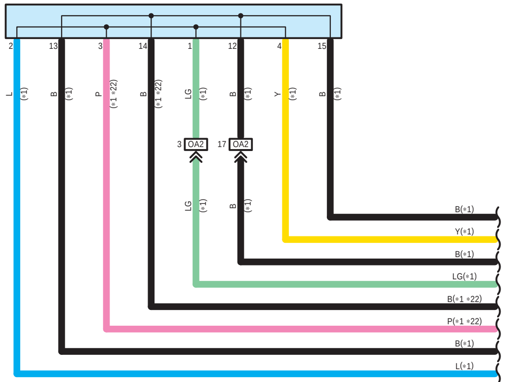
O196 No. 15 CAN Junction Connector
