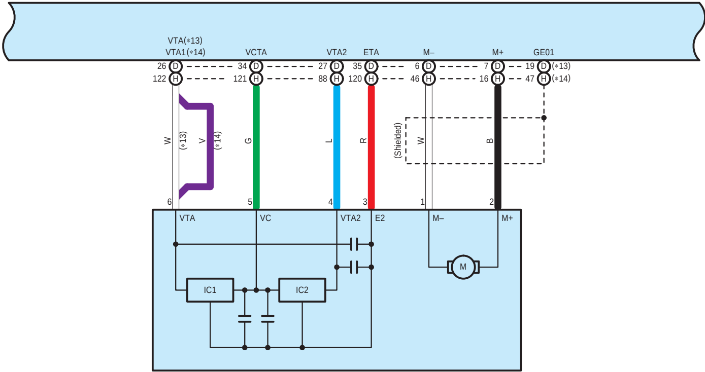
F21 Throttle Body with Motor Assembly
