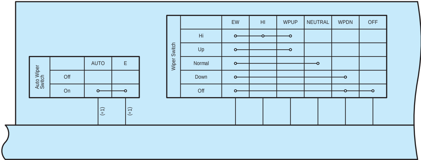
O23(A), O24(B), (C) Windshield Wiper Switch Assembly
