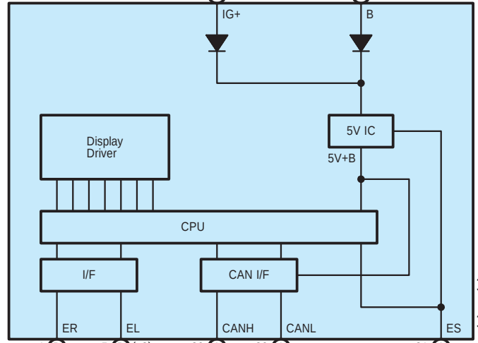
O3(A), O4(B) Combination Meter Assembly
