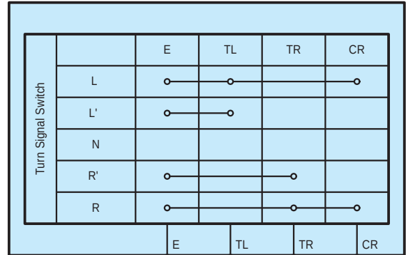
O22(A), (B) Headlight Dimmer Switch Assembly
