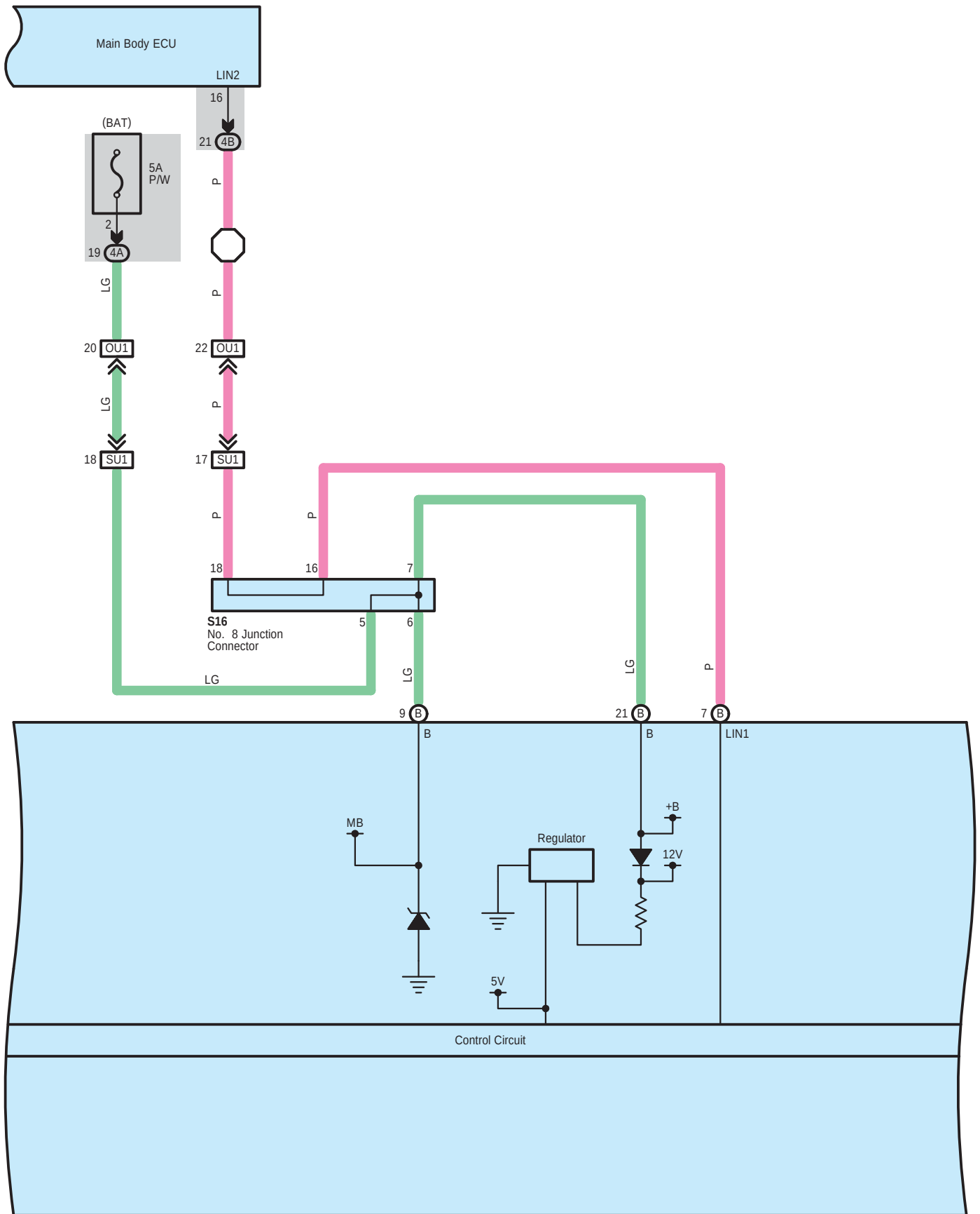
S10(B) Multiplex Network Master Switch Assembly
