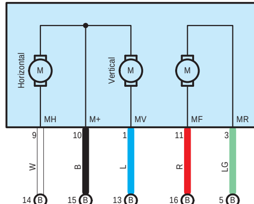
R7 Outer Rear View Mirror Assembly RH
