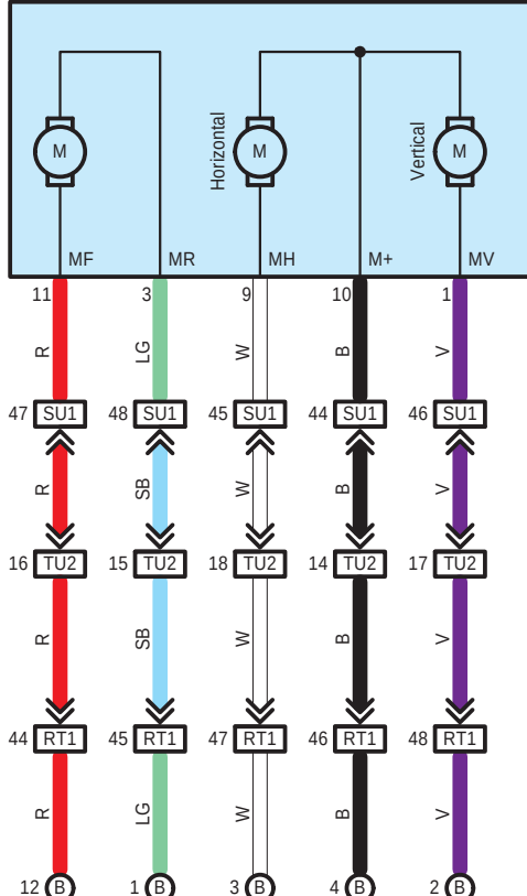
S7 Outer Rear View Mirror Assembly LH
