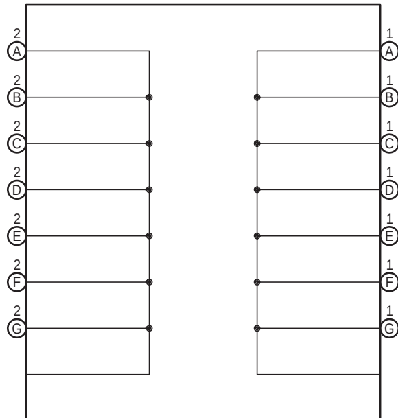
F73(A), F74(B), F75(C), F76(D), F77(E), F78(F), F87(G) Junction Connector
