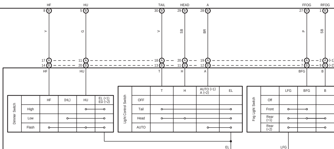
F39(A), F82(B) Headlight Dimmer Switch Assembly
