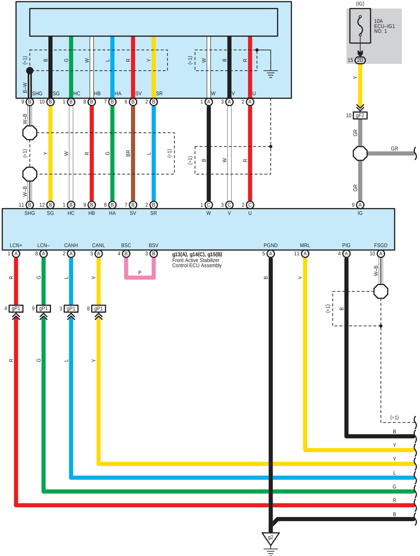
g16(A), g17(B) Front Active Stabilizer Control Actuator Assembly
