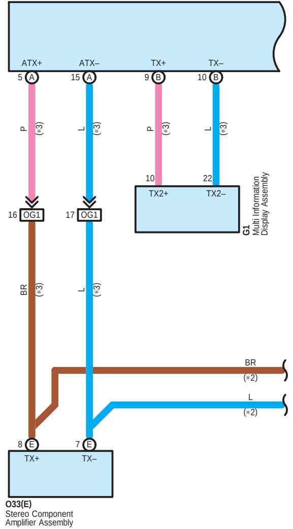
G7(A), G9(B), G11(D) Radio Receiver Assembly
