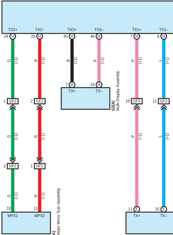
G35(H) Navigation Receiver Assembly
