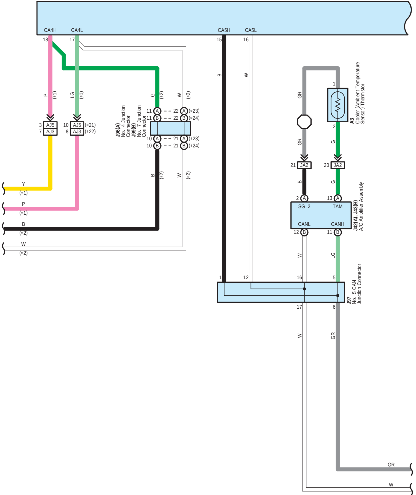
J75 Network Gateway ECU
