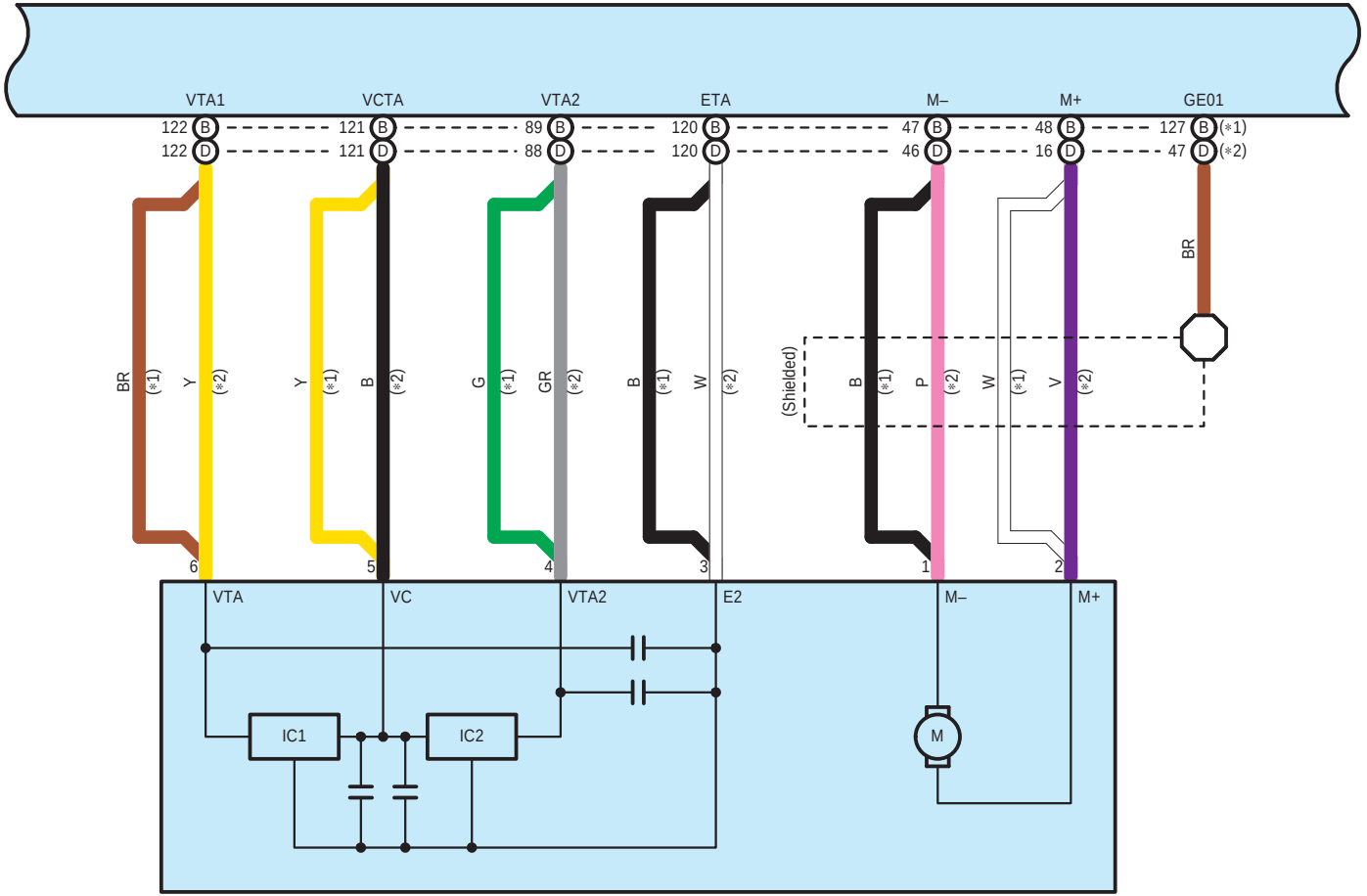
D37 Throttle Body with Motor Assembly
