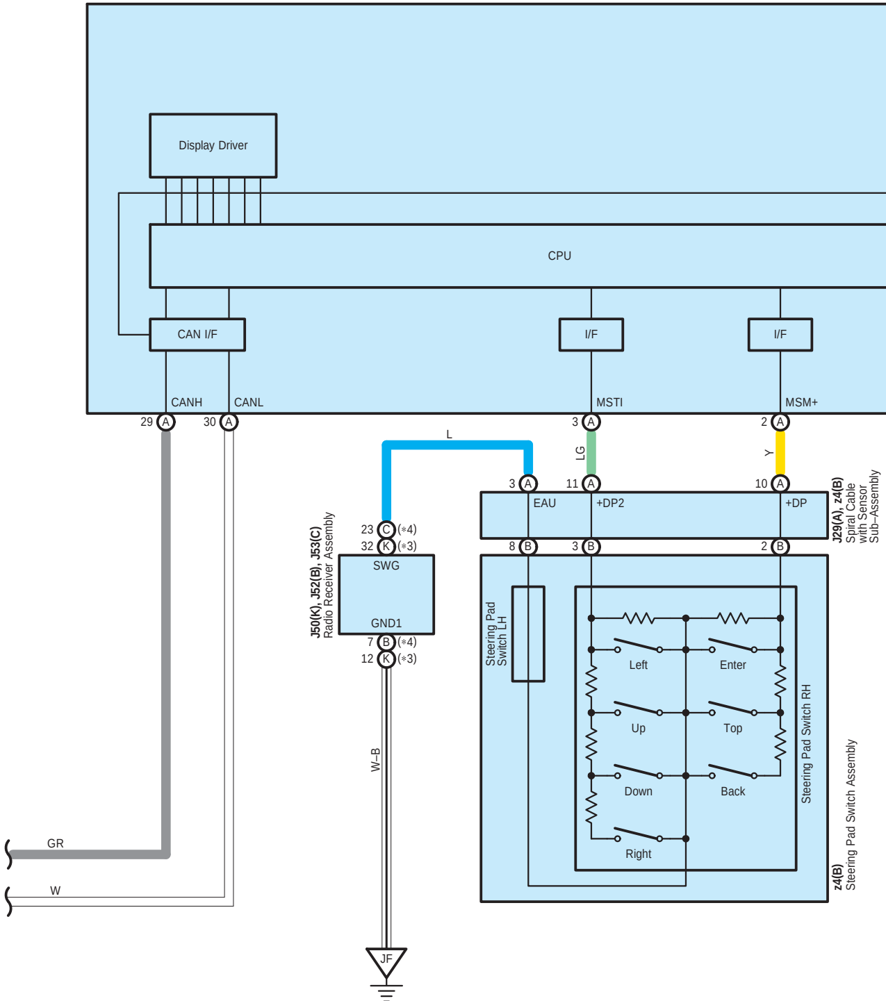
J10(A) Combination Meter Assembly
