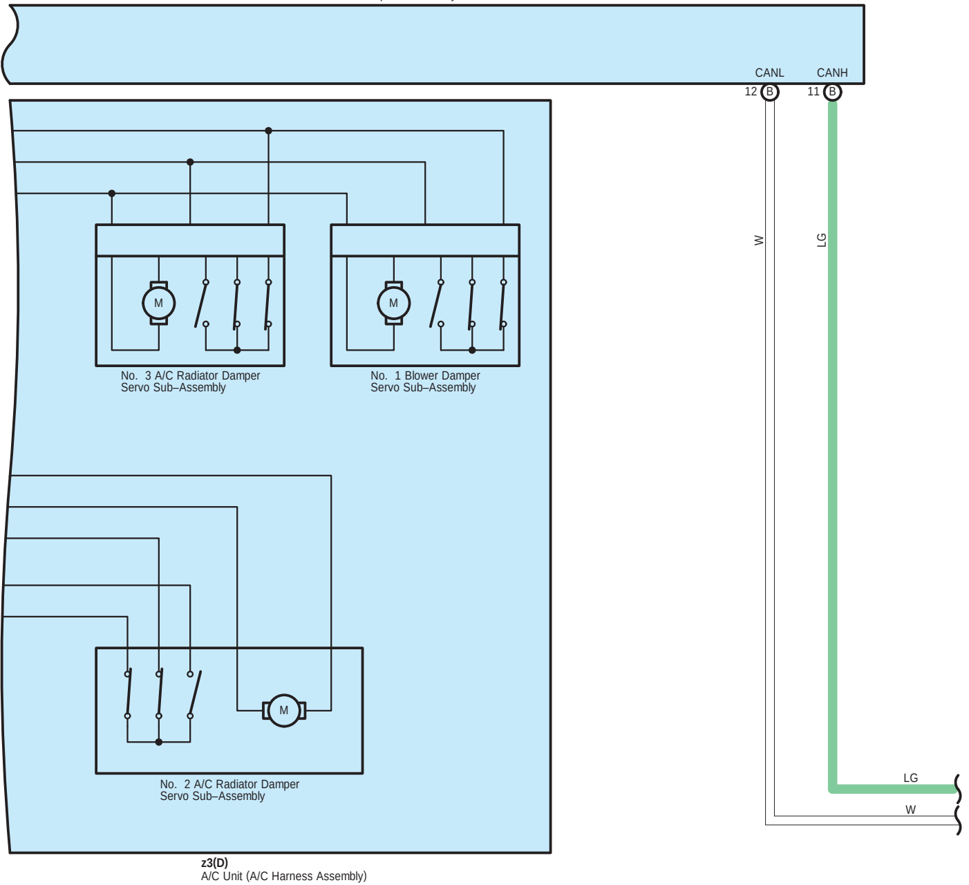
J42(A), J43(B), J48(C), z3(D) A/C Amplifier Assembly
