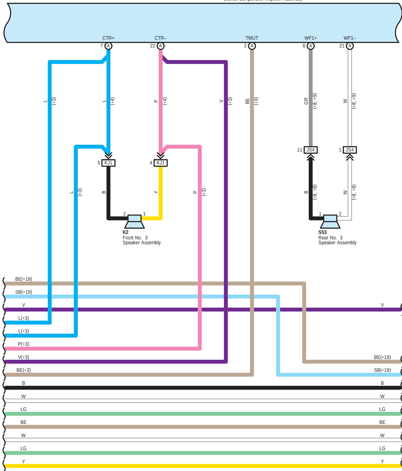
J66(A), J123(B) Stereo Component Amplifier Assembly
