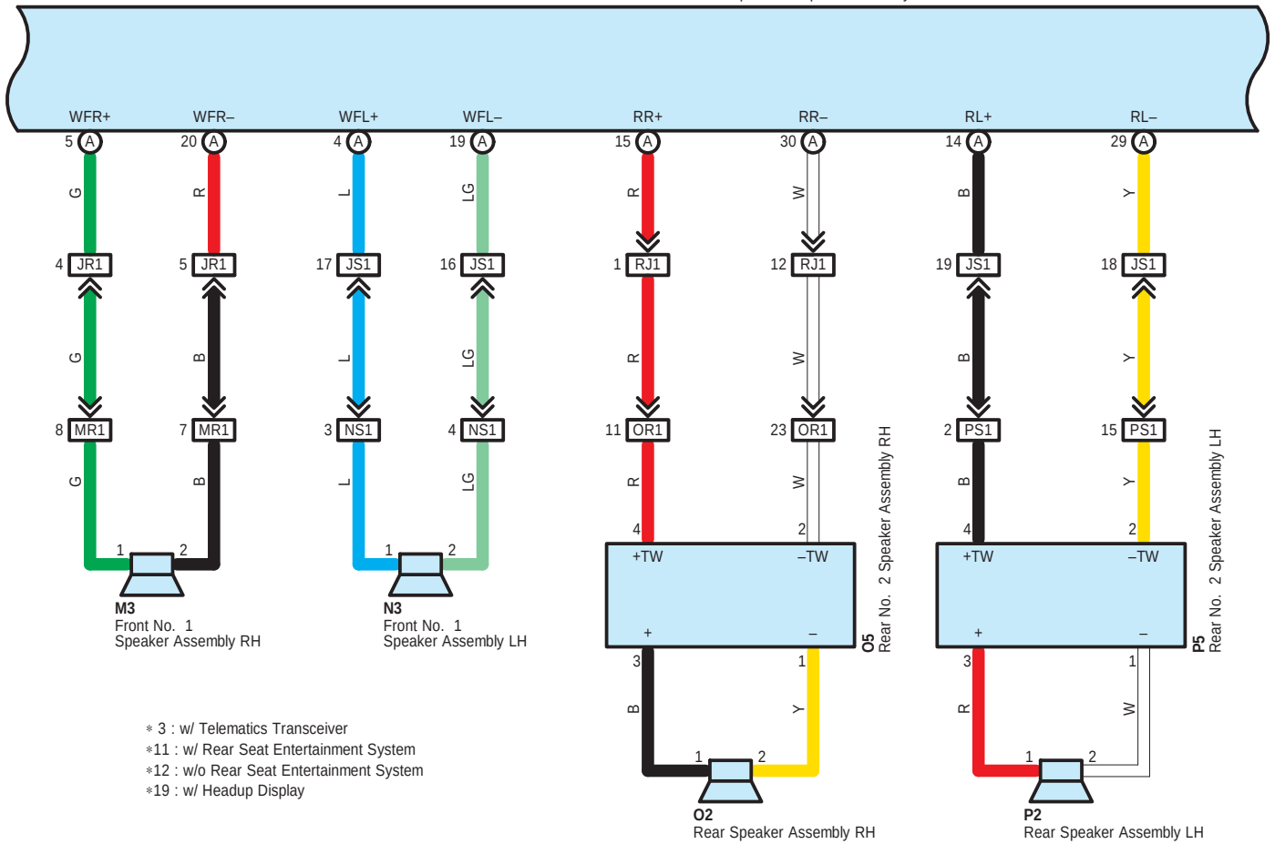
J66(A), J123(B) Stereo Component Amplifier Assembly
