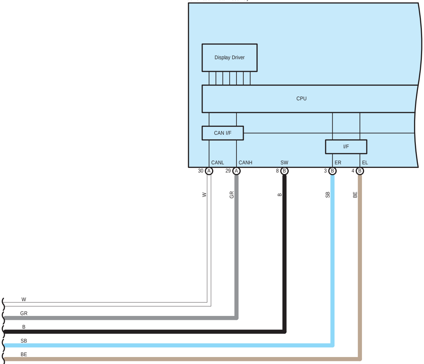
J10(A), J11(B) Combination Meter Assembly
