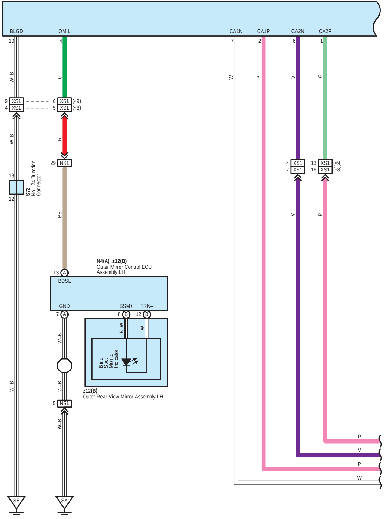
X2 Blind Spot Monitor Sensor LH
