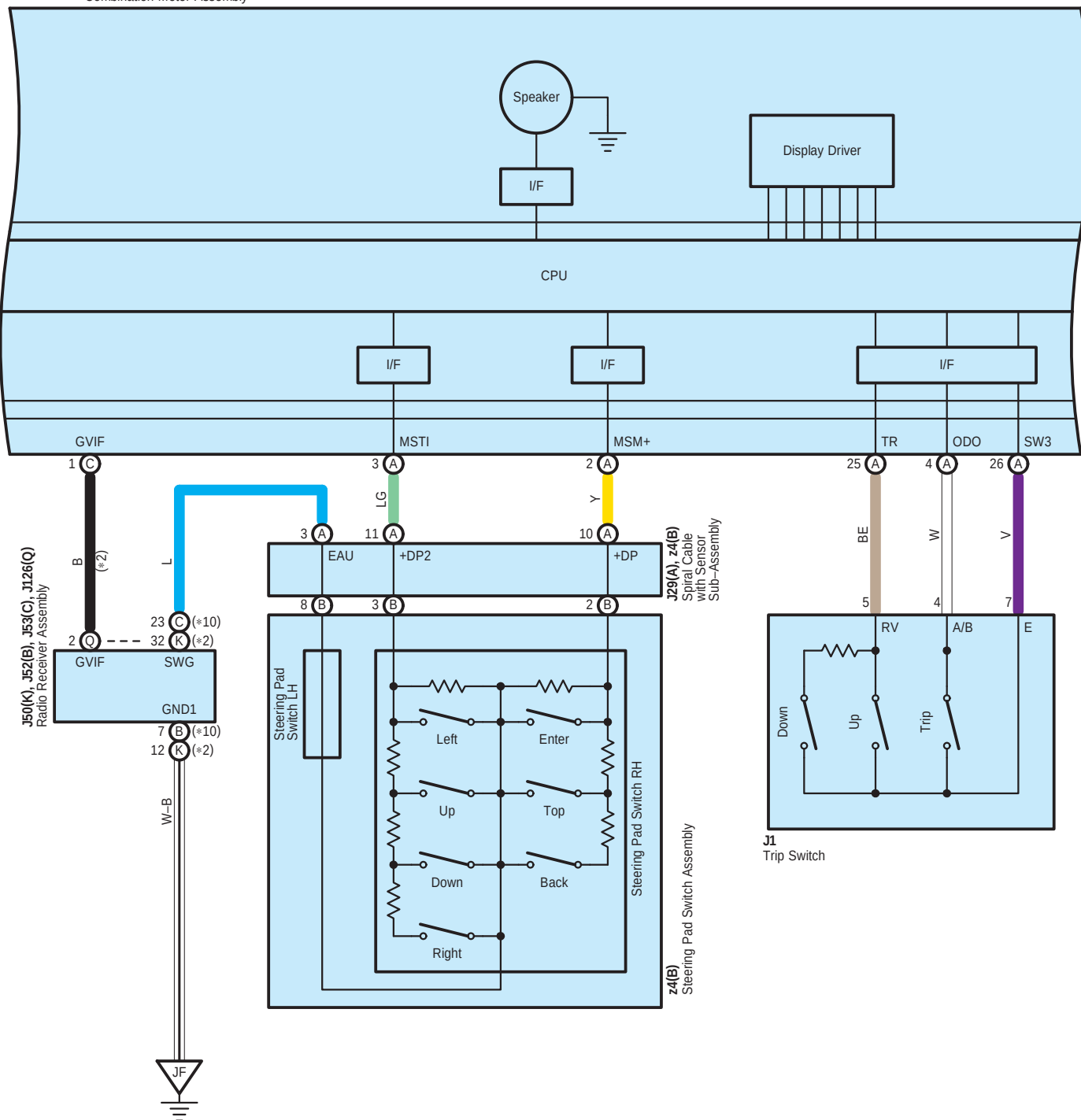
J10(A), J11(B), J127(C) Combination Meter Assembly
