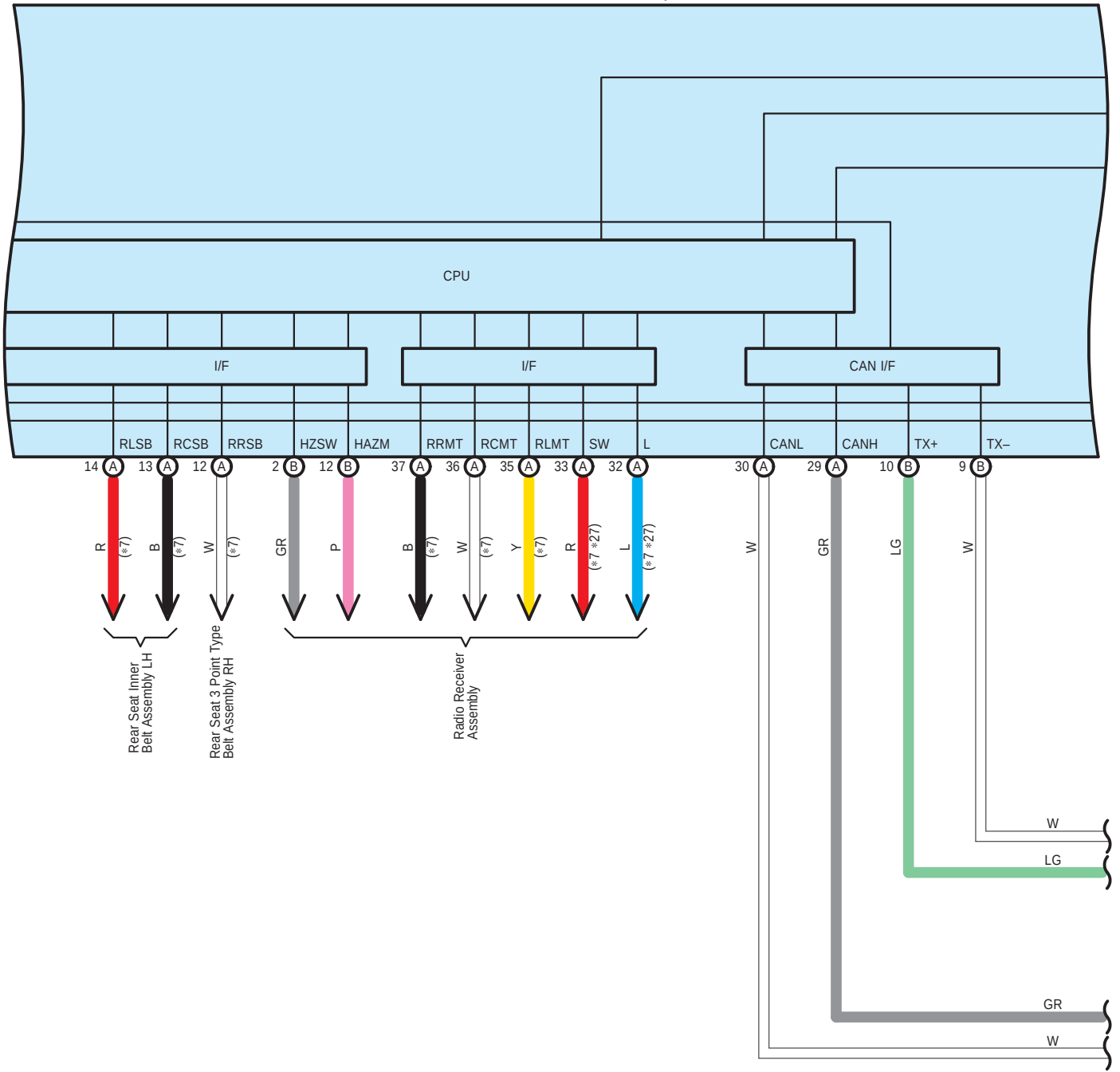
J10(A), J11(B), J127(C) Combination Meter Assembly
