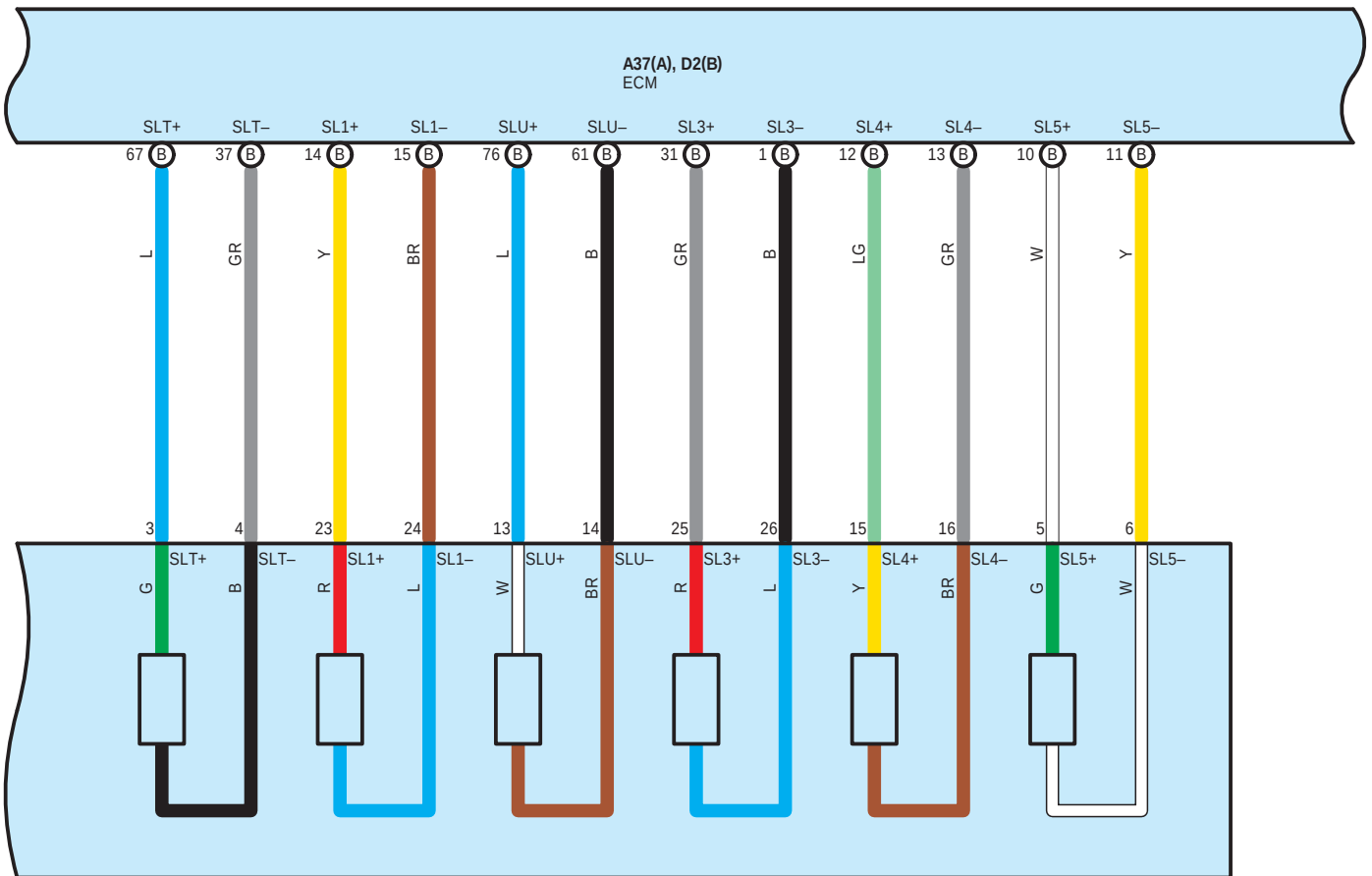
D56 ECT Solenoid (Transmission Wire)
